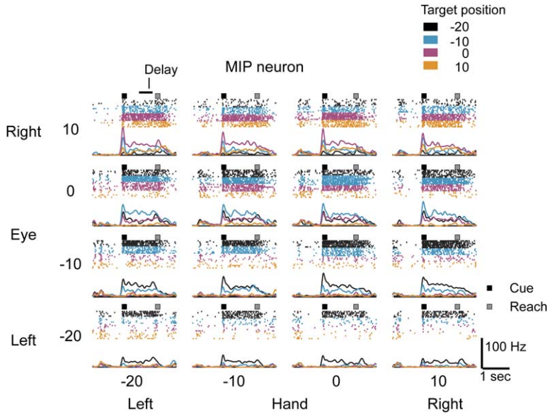
Figure 5. Example MIP Cell
