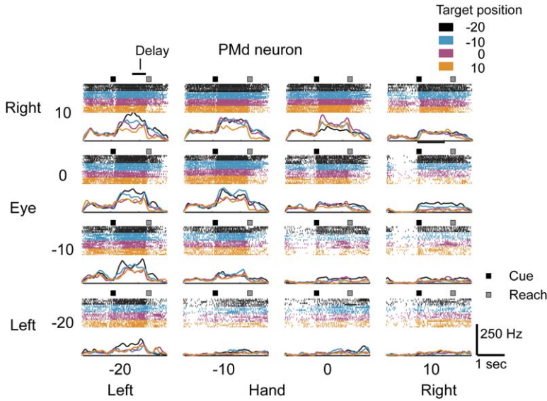
Figure 3. Example PMd Cell Responses to the reference frame dissociation task are aligned to target onset (black square) as eye position is varied (rows), hand position is varied (columns), and target position is varied (within each panel). Eye (E), hand (H), and target (T) positions are shown above each panel. Spike rasters are shown above the panel color-coded for each target position in that panel. Target onset time (black square) and mean movement onset time (gray square) are shown on each panel. The horizontal bar on the top left panel indicates the delay period analysis interval.
