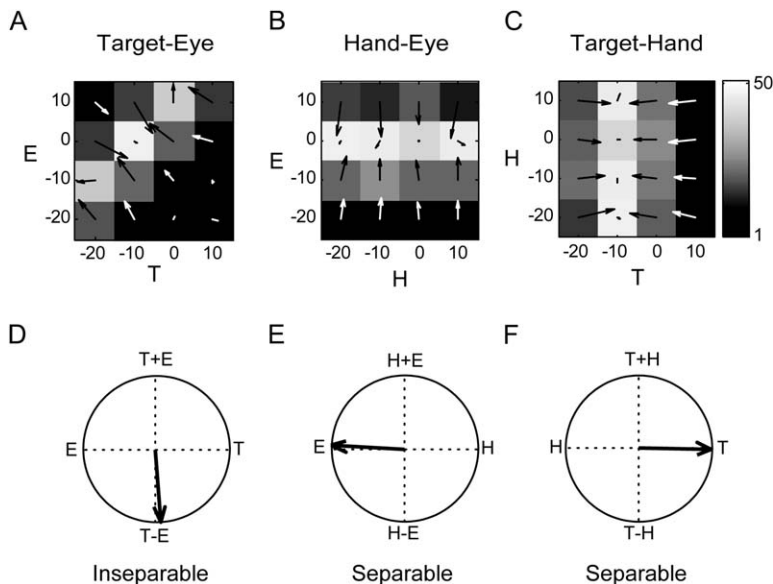
Figure 6. Example MIP Cell Eye-Hand-Target Response Matrices
