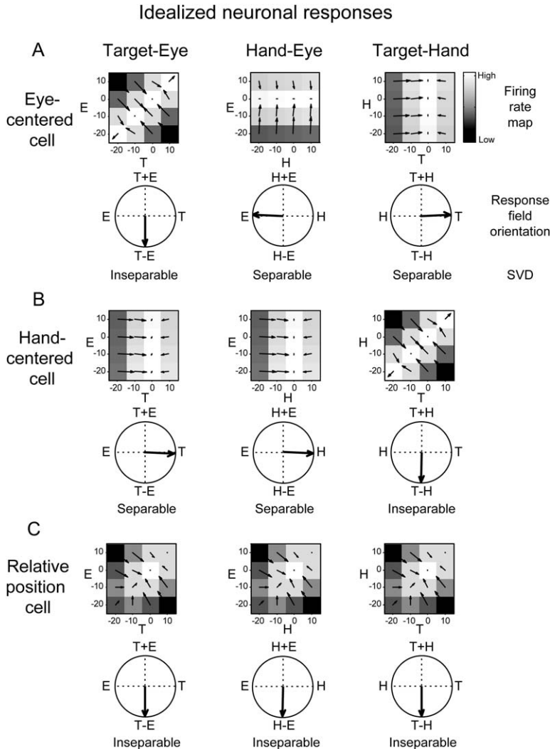
Figure 2. Idealized Cell Responses with Eye-Hand-Target Tuning for Cells with Three Different Reference Frames
