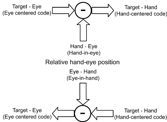
Figure 8. Schematic for Invertible Transformations Schematic showing how a relative position code performs invertible sensory-motor transformations between eye-centered and hand-centered reference frames.
