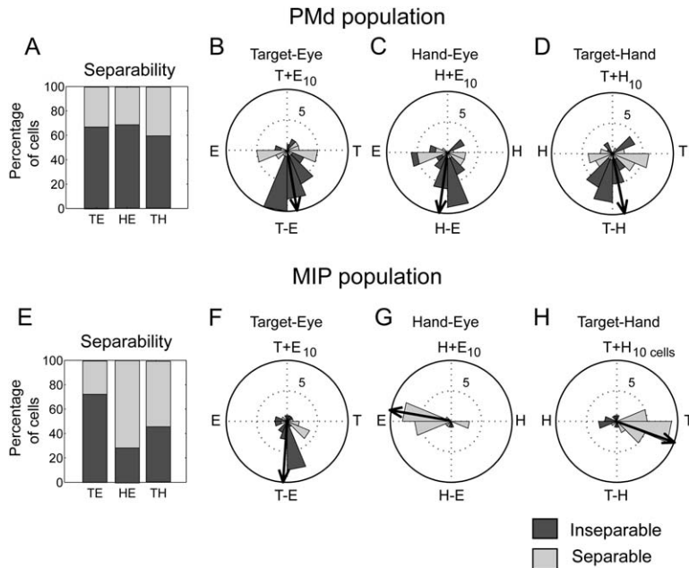
Figure 7. Population Eye-Hand-Target Analysis during the Delay Period
