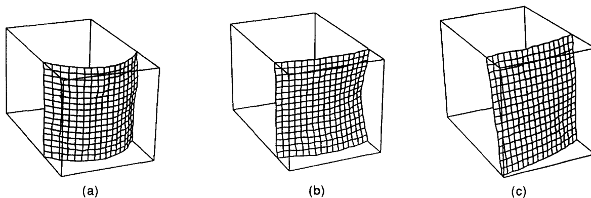
FIGURE 4. Degradation of the surface interpolation process for fewer points. A set of points in depth are first sampled from the surface of a cylinder and locations at which no explicit depth information is given are initially assigned a depth that is roughly the average of the known points. (a) The solution obtained after 50 iterations of the surface interpolation algorithm, for the case where 60 points are placed on a grid of size 17 \times 17 elements. (b) The solution obtained after the same number of iterations, for the case of 6 points. (c) The solution obtained for a set of 6 points whose positions are skewed toward one side of the cylinder.
