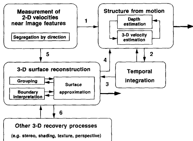
FIGURE 1. Diagram of a model that combines 2-D motion measurement, recovery of 3-D structure from motion, temporal integration and surface reconstruction. See text for details.
