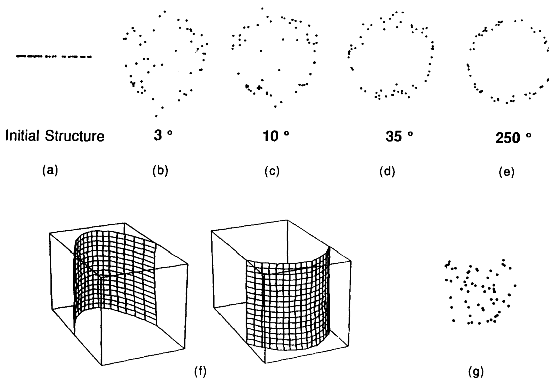
FIGURE 2. Example of the temporal buildup of 3-D structure from motion. 60 points were randomly positioned on the surface of a cylinder and rotated 1^\circ per frame. Gaussian distributed noise was added to the image velocities of the points, with the space constant of the Gaussian, \sigma = 0.5 , yielding an average relative error of 20% in the velocity components. After each rotation of the points, the depth and 3-D velocity computations were performed once, and roughly 60 iterations were performed within the 3-D velocity computation. (a) Bird's eye view of the initial flat solution. (b-e) The solution after 3^\circ , 10^\circ , 35^\circ and 250^\circ of total rotation, respectively. (f) The result of the surface approximation algorithm applied to the final depths shown in (e). Separate pictures are shown for the front and back surfaces. (g) The results of the structure-from-motion and temporal integration algorithms applied to the unstructured stimulus explored by Husain et al. (1989)
