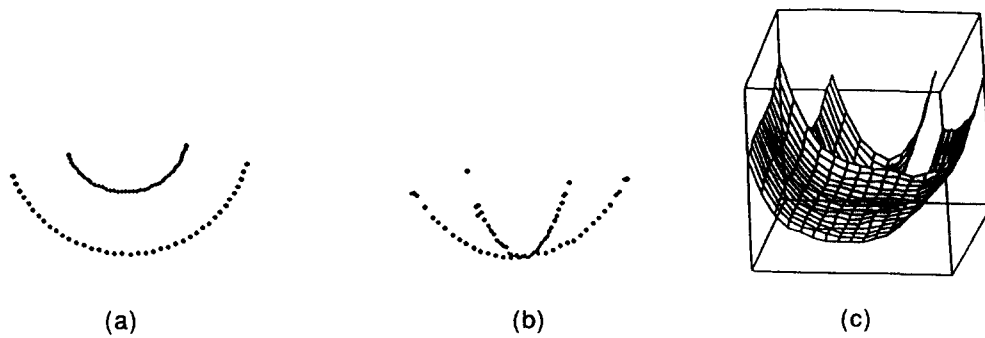
FIGURE 7. Simulations with the model applied to perceptual demonstrations of Ramachandran et al. (1988) shown in Fig. 5c and d. (a) Birds' eye view of the true 3-D structure. (b) The results of the structure-from-motion algorithm applied to two frames that are separated by 1^\circ of rotation of the points. (c) The results of the surface reconstruction stage.
