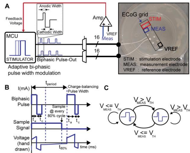
Fig. 3. A. Schematic of the active charge-balancing circuit. The increased voltage at measurement electrode ( V_{MEAS} ) activates the adaptive removal of residual charges by pulse width-modulated correction. Right box: ECoG grid is placed on phantom brain tissue. Dipole channels in 6x2 ECoG grid are stimulated bipolarly. Charge accumulation was tracked in the neighboring electrode from the stimulation pairs. The reference voltage was defined from the most distant electrode in the grid. B. Illustration of a biphasic pulse waveform and the timing of the voltage measurement ( V_{MEAS} ). C. Binary state machine algorithm to test the active charge balancing. The output of each state differs in their ratio between the anodic and cathodic pulse width (either 12:1 or 1:12). V_{TH} : pre-configured threshold voltage.
