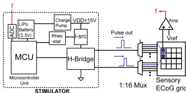
Fig. 2. Schematic of the stimulator circuit. The output pulses are current-controlled, biphasic pulses with programmable pulse width, pulse frequency, and charge density. MCU: microcontroller. ADC: analog-to-digital converter. I-src: current source. Vref: reference voltage. Mux: Multiplexer. f: feedback voltage.
