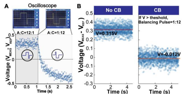
Fig. 5. A. Transient voltage response at the measurement electrode to the switching of the pulse output profile without the charge balancing mechanism: 1) Anodic vs Cathodic=12:1, 2) Anodic vs Cathodic=1:12. B. The effect of charge-balancing. Measured steady-state voltage is 0.315 \pm 0.048 when there is no charge-balancing, and -0.012 \pm 0.052 when there is active charge balancing. The voltage is measured once per each cycle as in Fig. 3B. CB: Charge-Balancing. *Each dot represents a voltage sample taken at 80% of each duty cycle of the 200 Hz pulse train.
